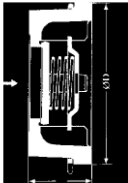
Centering ring DN15 to DN100
